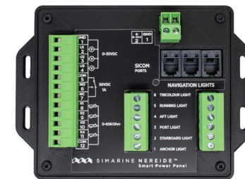
STP06 Navigation Light and Tank Monitoring Module
